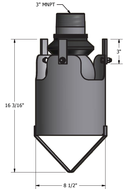
6" Stainless Steel Cage
