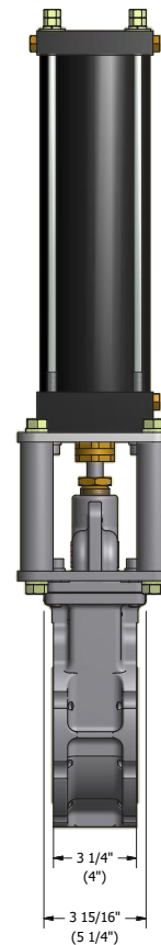
KEY: 4" VALVE DIMENSIONS (6" VALVE) DIMENSIONS
