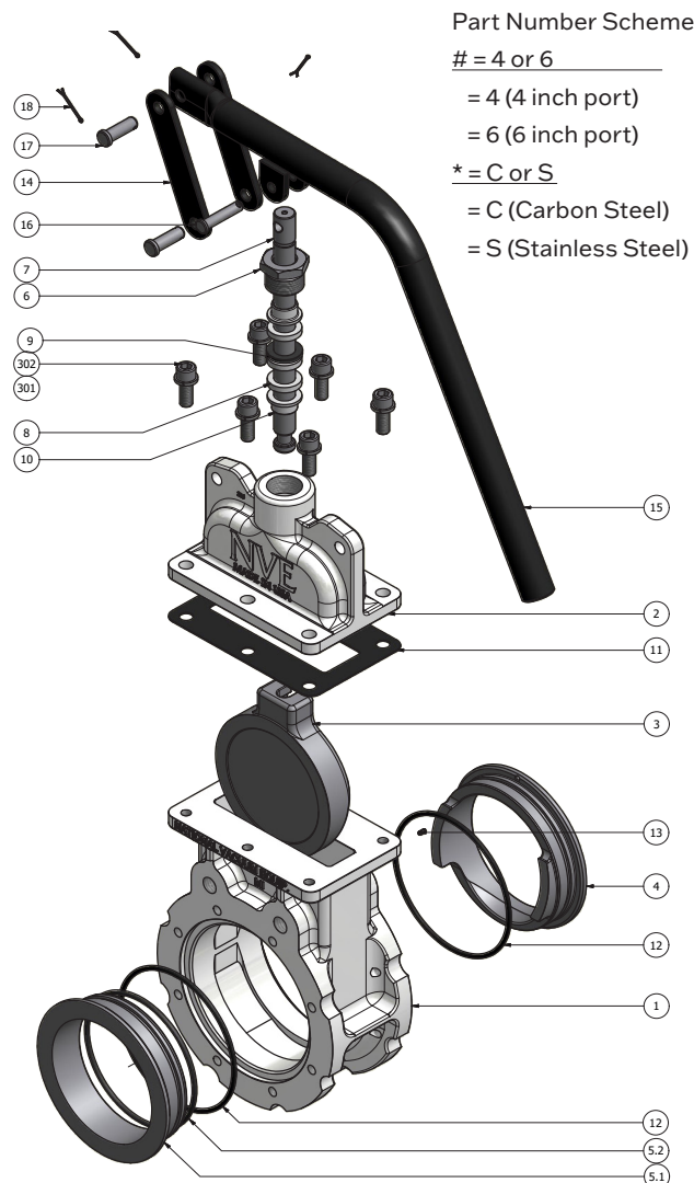
4 and 6 NVE Single Gate Valve Parts Diagram
